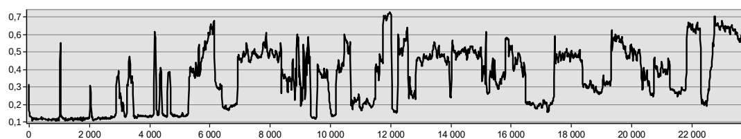
Fig. 6. Profile of NDVI index values for May 05 2018 on the territory of Razdolnensky district of the Republic of Crimea on the A-B line. Compiled by the author
